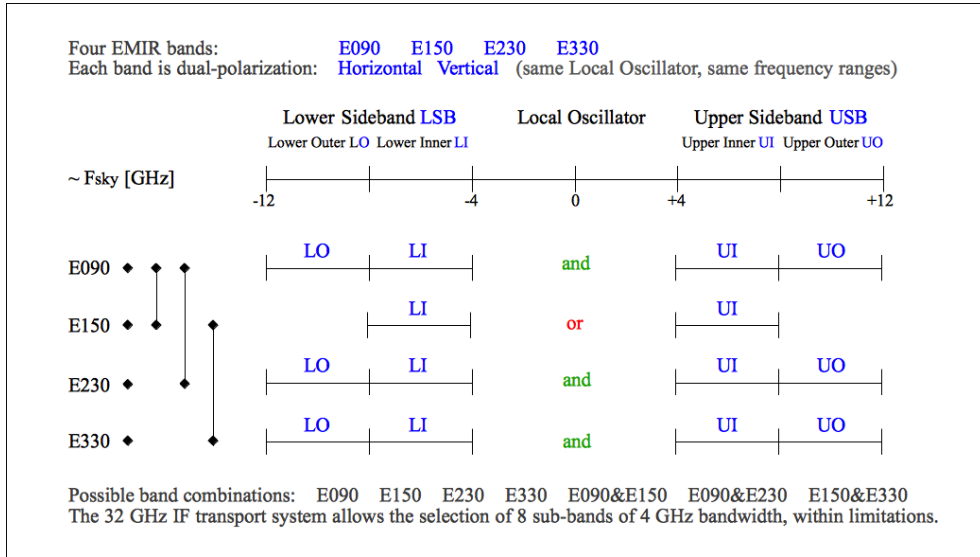
Figure 2: Visual overview of EMIR bands after the upgrade. Eight sub-bands can be transported to backends for a total of 32 GHz instantaneous bandwidth. Note that the frequencies indicated at the sideband edges should be considered as indications only since they will likely slightly change in the near future.
