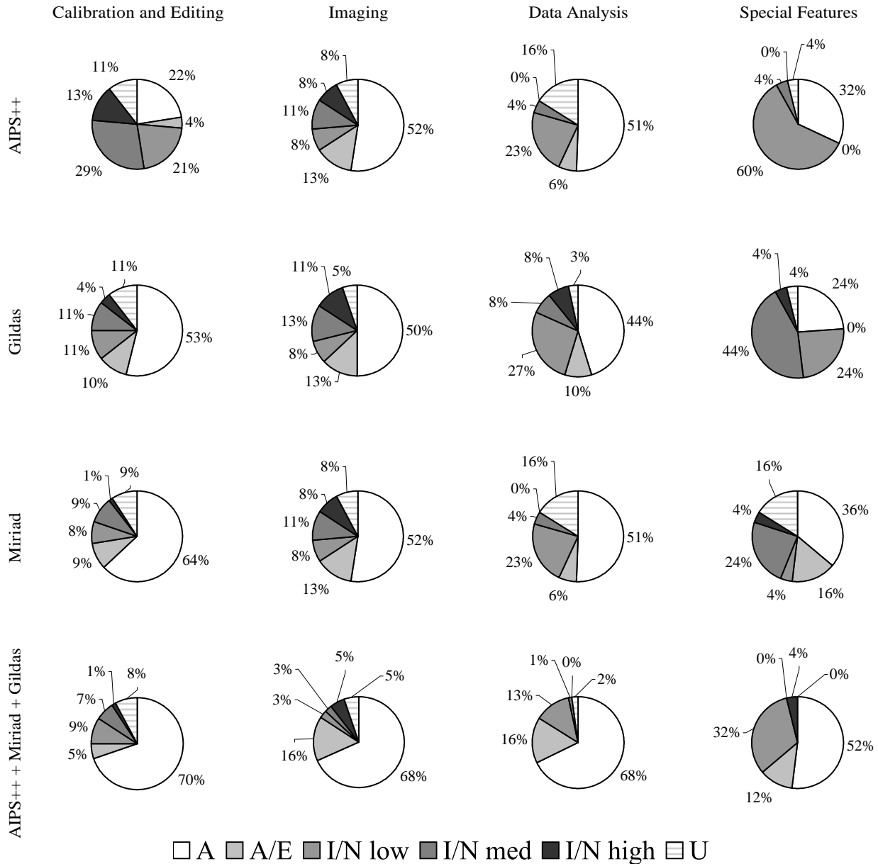
Figure 3: Same as Fig. 1 except that requirements are sorted by functionalities related to reduction steps: calibration and editing, imaging, data analysis and special features (Solar system, VLBI, pulsar). Critical, important and desirable features have the same weight.
