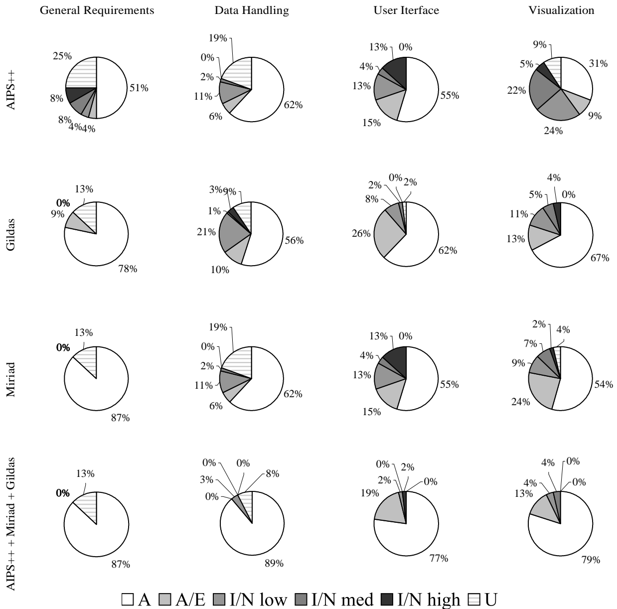
Figure 2: Same as Fig. 1 except that requirements are sorted by functionalities related to user interface: general requirements, data handling, user interface and visualization. Critical, important and desirable features have the same weight.
