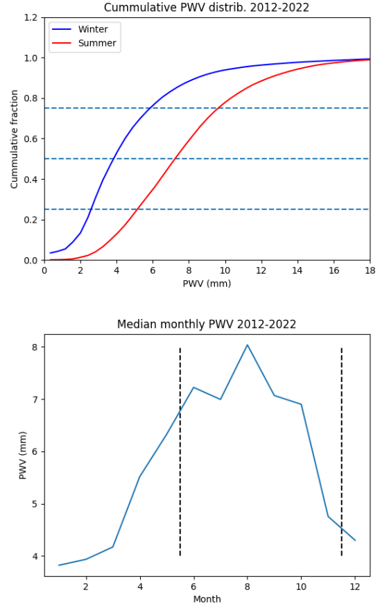
Figure 3: Amount of precipitable water vapor (pwv) derived from the 225 GHz taumeter at the 30-m observatory averaged over the years 2012 to 2022.
